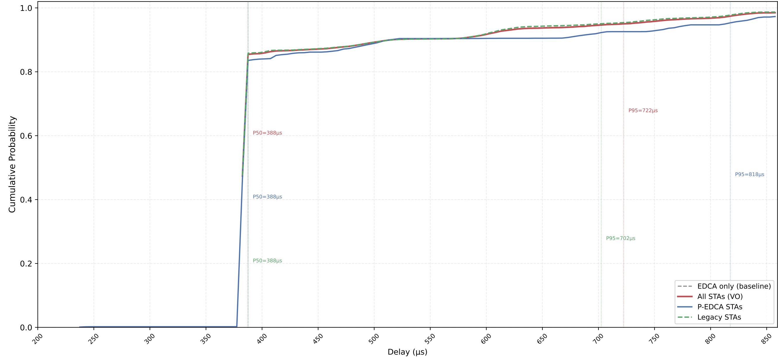
VO Delay CDF — P-EDCA / Legacy / All | CWds=1 × QSRC=1 × PSRC=3 nSta=30, nPedca=5/30, 0.1Mbps, avg of 10 runs
