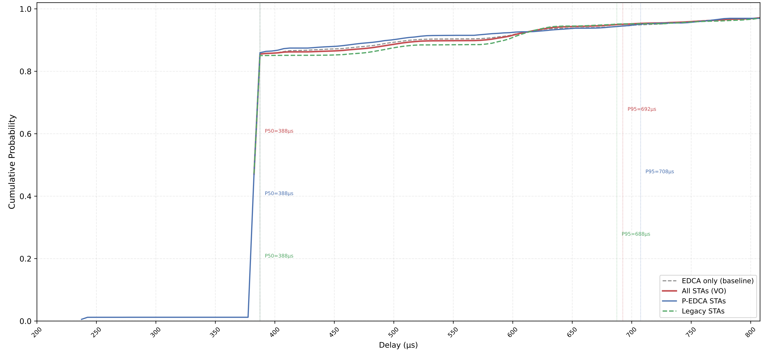
nSta=30, nPedca=15/30, 0.1Mbps, avg of 10 runs
