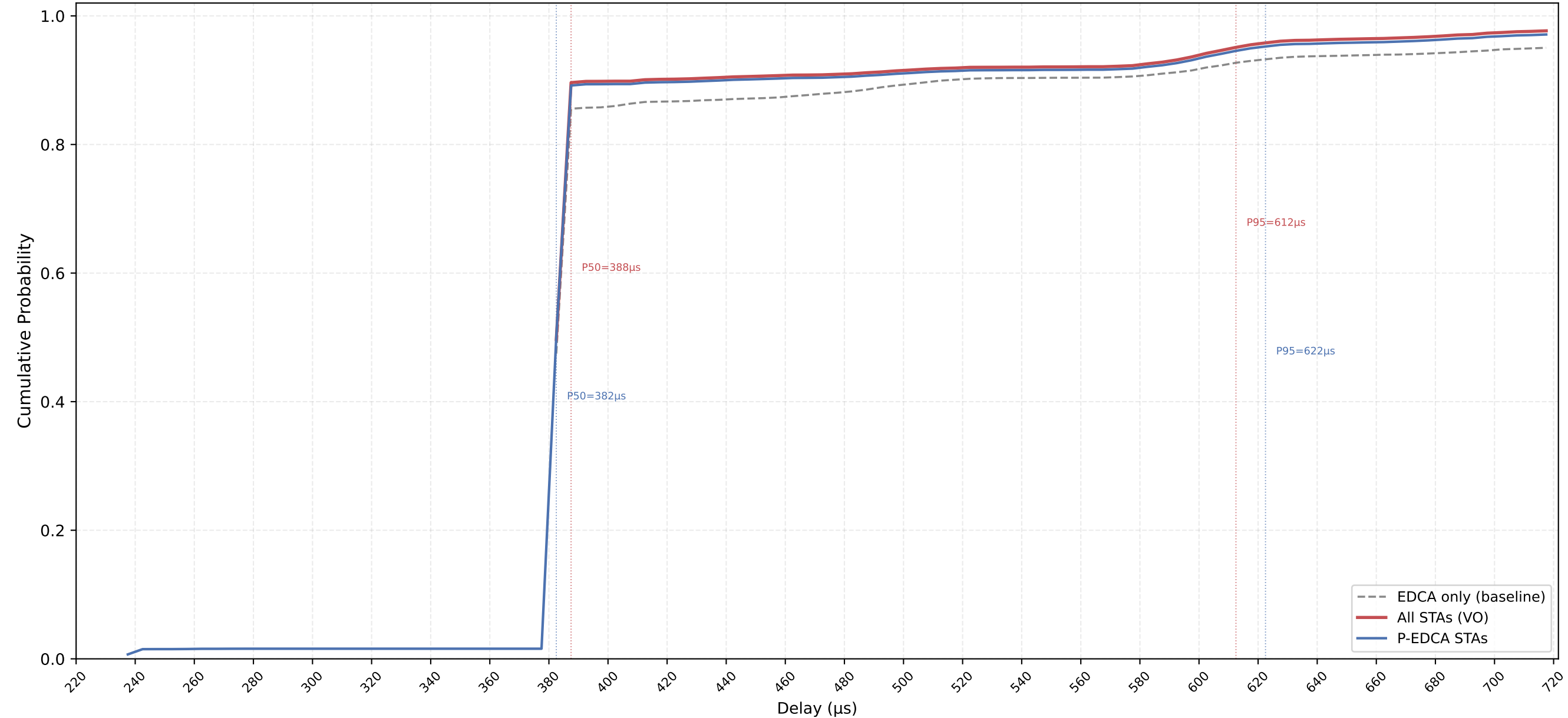
VO Delay CDF — P-EDCA / Legacy / All | CWds=1 × QSRC=1 × PSRC=3 nSta=30, nPedca=30/30, 0.1Mbps, avg of 10 runs
