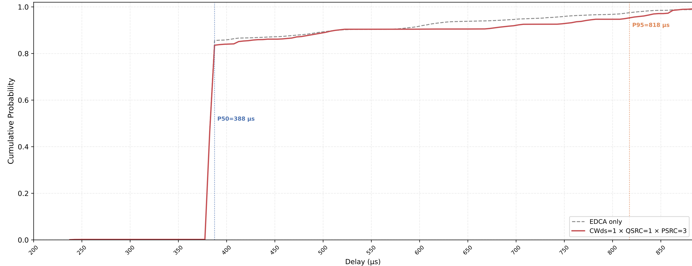
P-EDCA STA VO Delay CDF — CWds=1 × QSRC=1 × PSRC=3 nSta=30, nPedca=5, 0.1Mbps, avg of 10 runs
