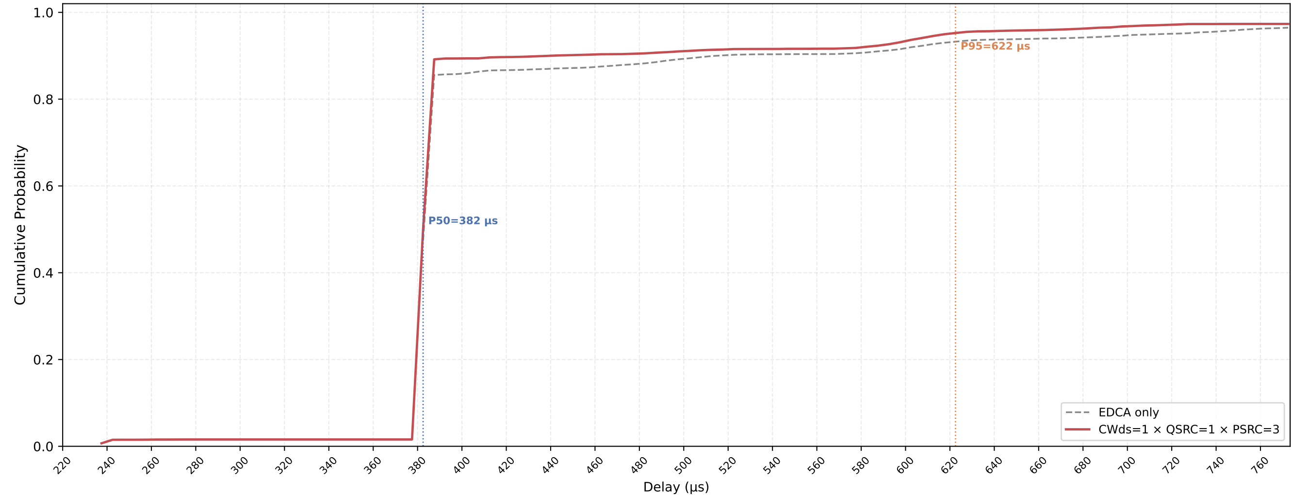
P-EDCA STA VO Delay CDF — CWds=1 × QSRC=1 × PSRC=3 nSta=30, nPedca=30, 0.1Mbps, avg of 10 runs
