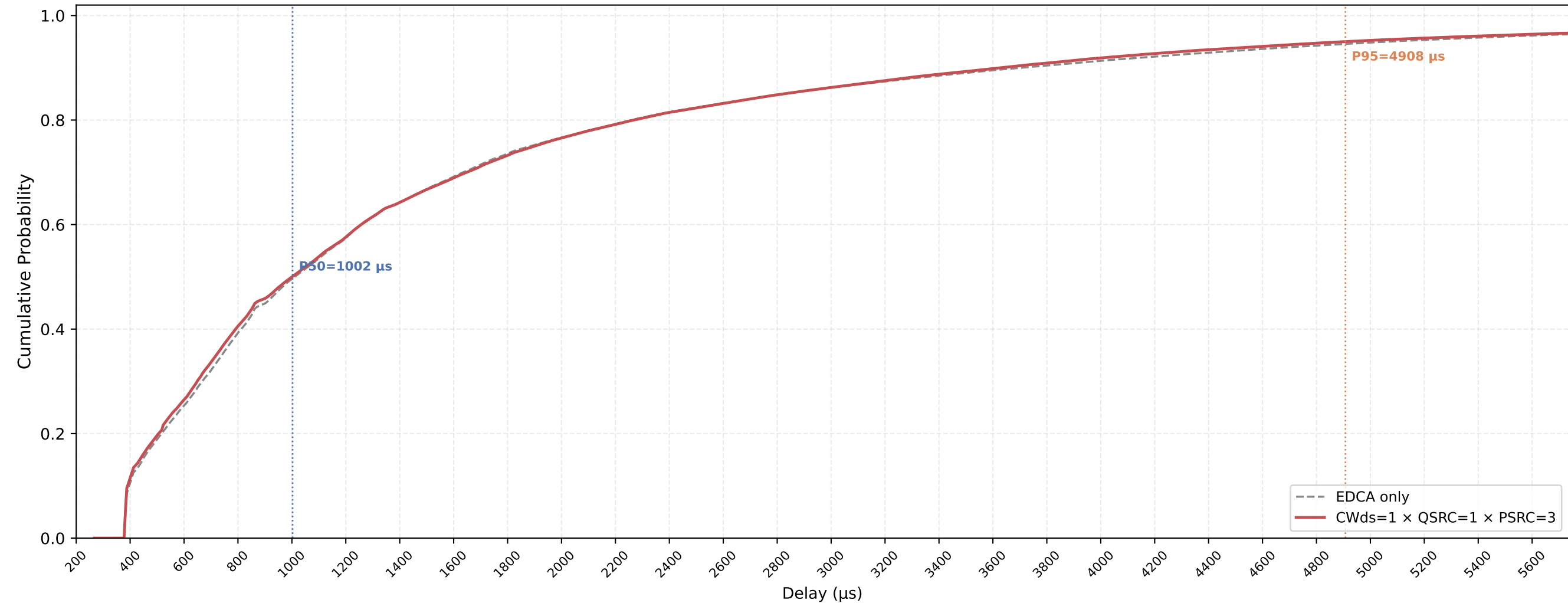
VO (all STAs) Delay CDF — CWds=1 × QSRC=1 × PSRC=3 nSta=30, nPedca=5, 0.5Mbps, avg of 10 runs
