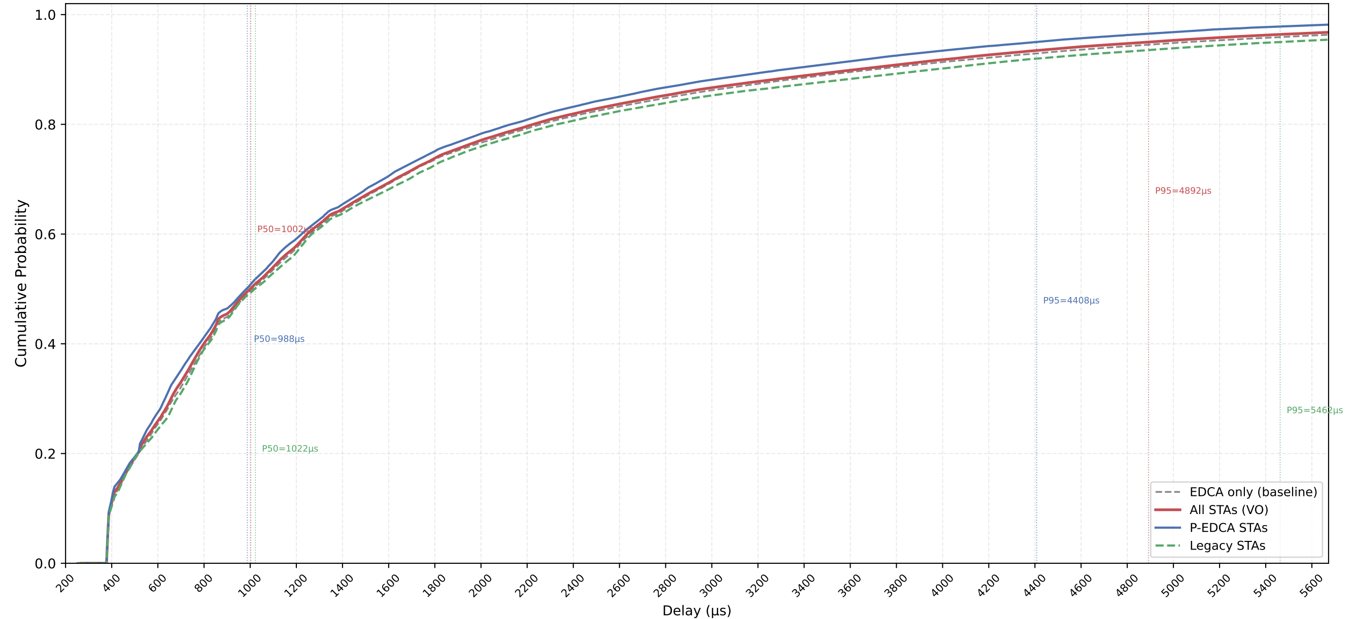
VO Delay CDF — P-EDCA / Legacy / All | CWds=1 × QSRC=2 × PSRC=1 nSta=30, nPedca=15/30, 0.5Mbps, avg of 10 runs
