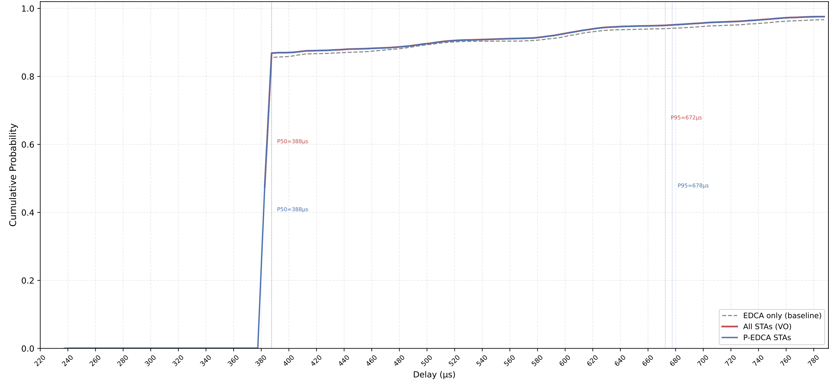
VO Delay CDF — P-EDCA / Legacy / All | CWds=1 × QSRC=2 × PSRC=1 nSta=30, nPedca=30/30, 0.1Mbps, avg of 10 runs
