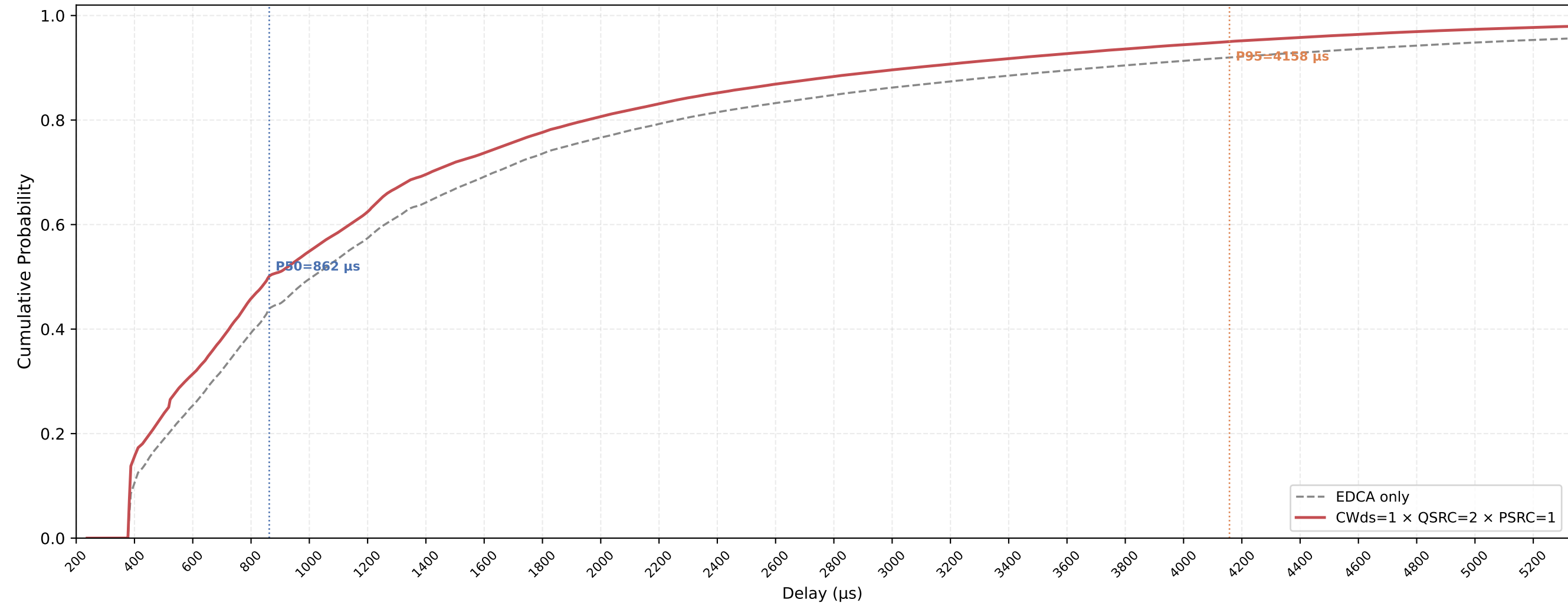
P-EDCA STA VO Delay CDF — CWds=1 × QSRC=2 × PSRC=1 nSta=30, nPedca=30, 0.5Mbps, avg of 10 runs
