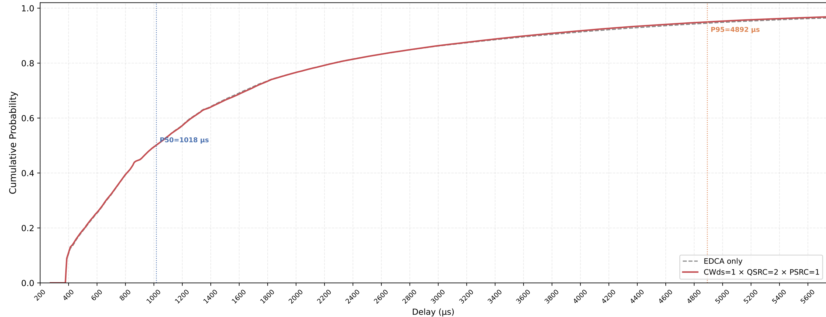
VO (all STAs) Delay CDF — CWds=1 × QSRC=2 × PSRC=1 nSta=30, nPedca=5, 0.5Mbps, avg of 10 runs
