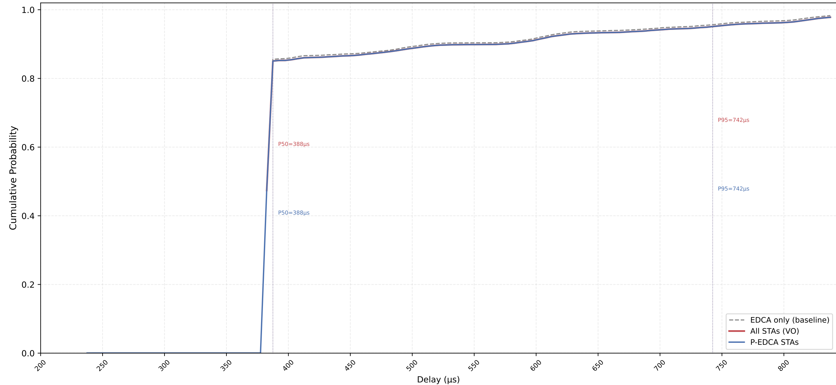
VO Delay CDF — P-EDCA / Legacy / All | CWds=1 × QSRC=2 × PSRC=2 nSta=30, nPedca=30/30, 0.1Mbps, avg of 10 runs
