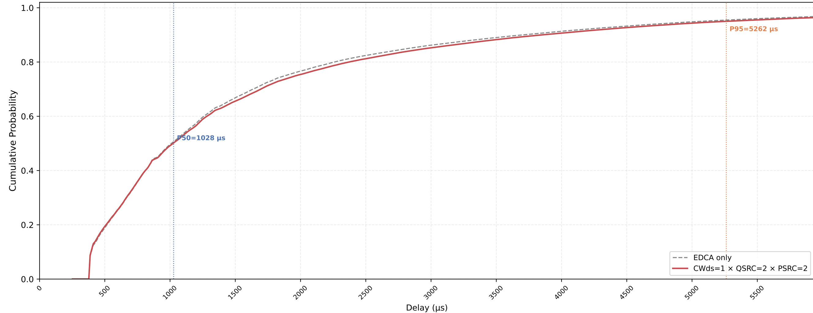
Legacy STA VO Delay CDF — CWds=1 × QSRC=2 × PSRC=2 nSta=30, nPedca=5, 0.5Mbps, avg of 10 runs
