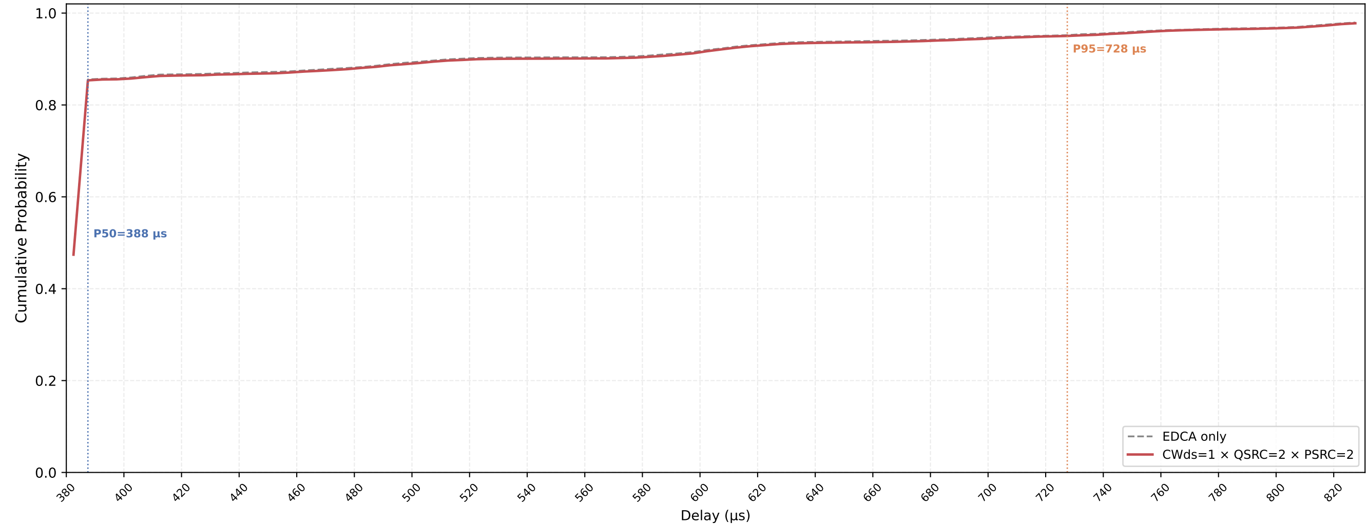
VO (all STAs) Delay CDF — CWds=1 × QSRC=2 × PSRC=2 nSta=30, nPedca=15, 0.1Mbps, avg of 10 runs
