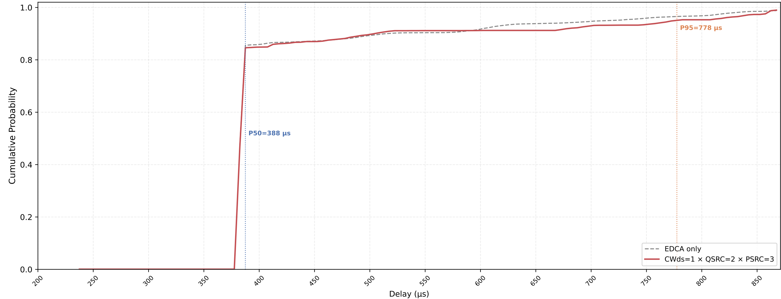
P-EDCA STA VO Delay CDF — CWds=1 × QSRC=2 × PSRC=3 nSta=30, nPedca=5, 0.1Mbps, avg of 10 runs
