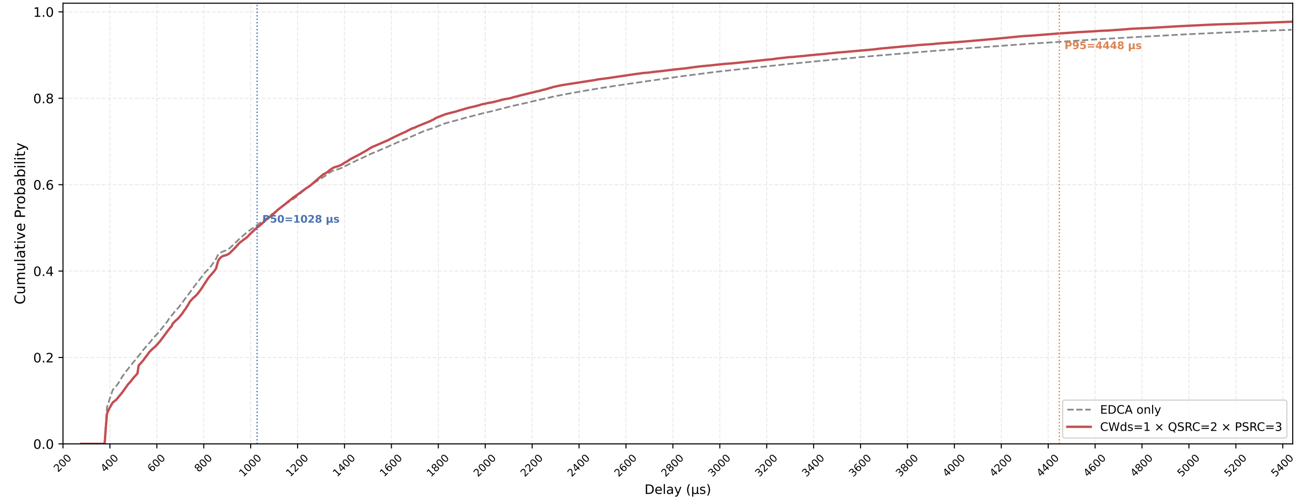
P-EDCA STA VO Delay CDF — CWds=1 × QSRC=2 × PSRC=3 nSta=30, nPedca=5, 0.5Mbps, avg of 10 runs
