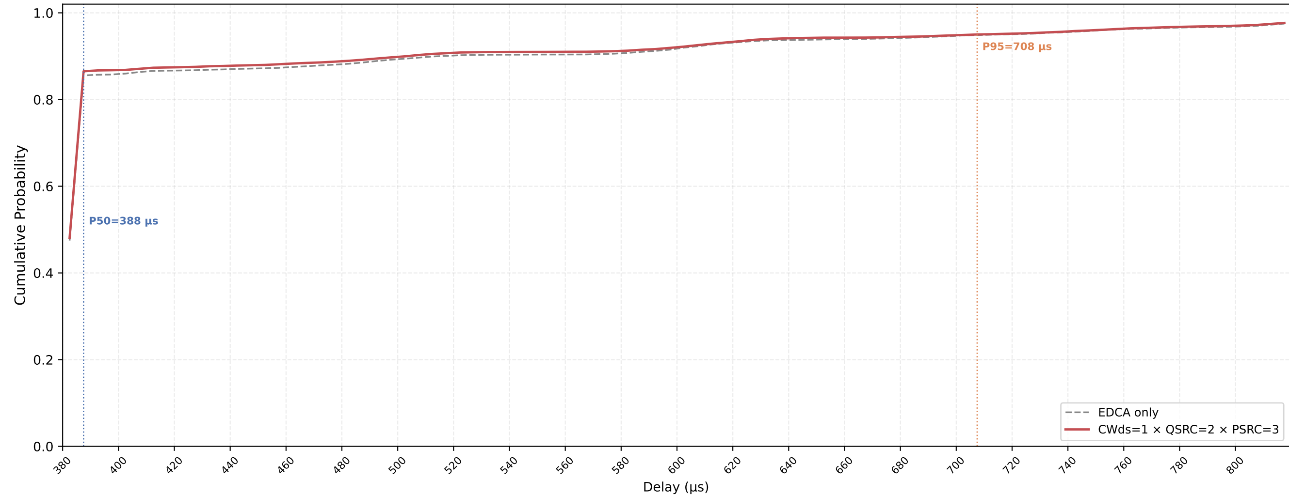
VO (all STAs) Delay CDF — CWds=1 × QSRC=2 × PSRC=3 nSta=30, nPedca=15, 0.1Mbps, avg of 10 runs
