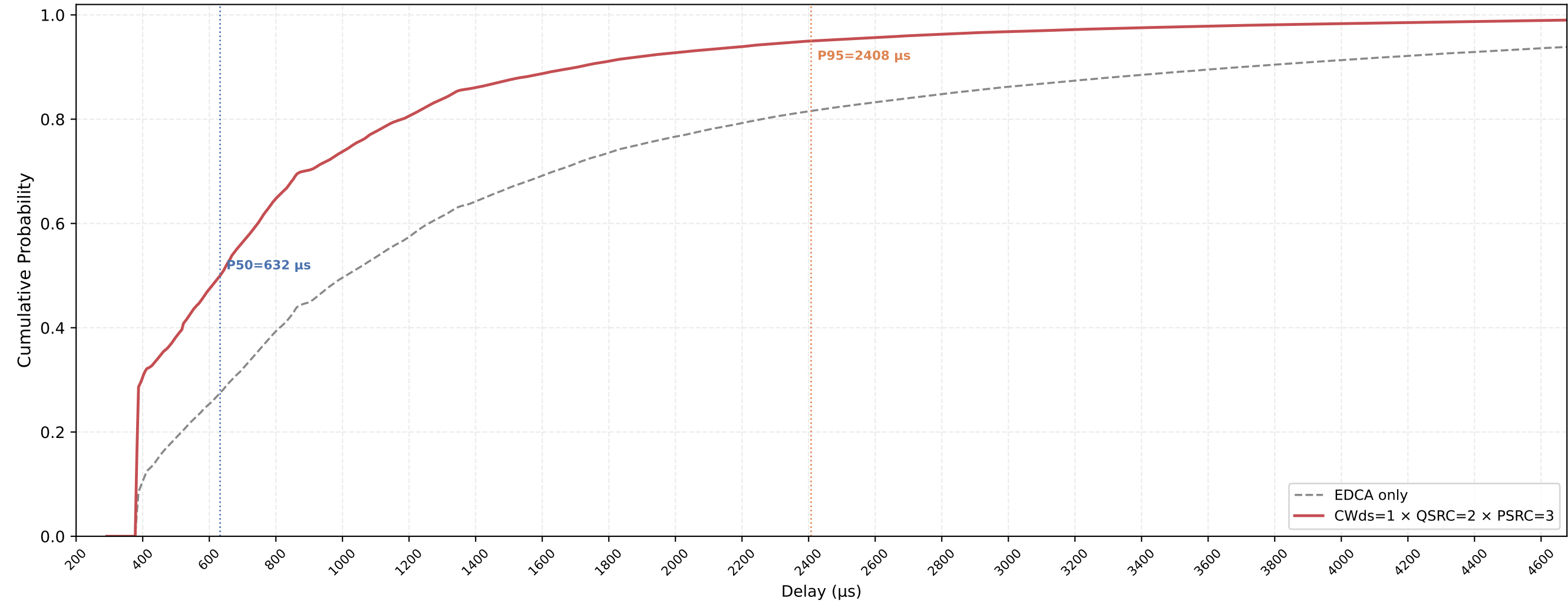
VO (all STAs) Delay CDF — CWds=1 × QSRC=2 × PSRC=3 nSta=30, nPedca=30, 0.5Mbps, avg of 10 runs
