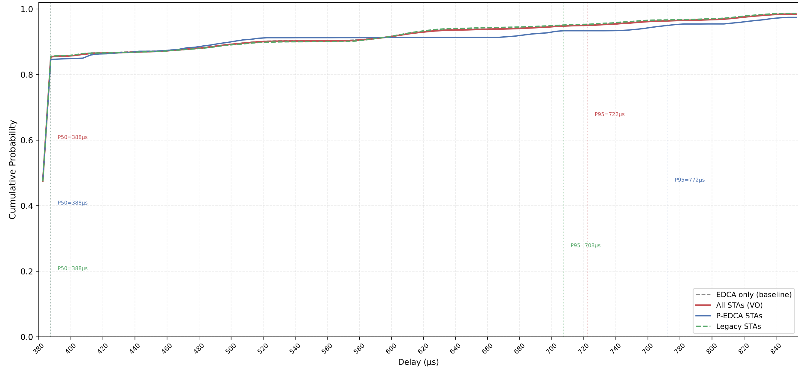
VO Delay CDF — P-EDCA / Legacy / All | CWds=1 × QSRC=3 × PSRC=1 nSta=30, nPedca=5/30, 0.1Mbps, avg of 10 runs
