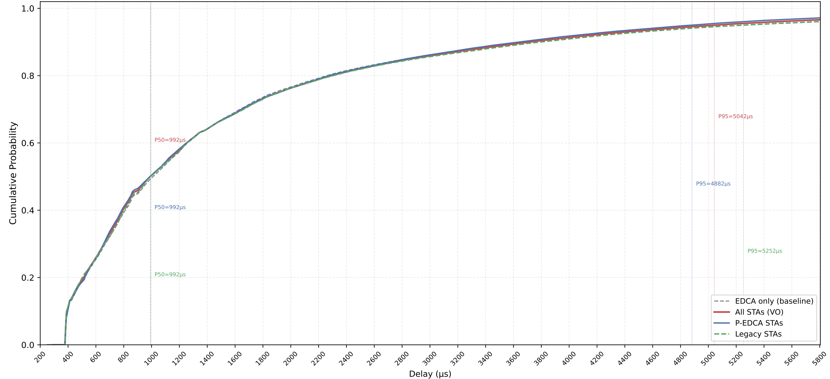
VO Delay CDF — P-EDCA / Legacy / All | CWds=1 × QSRC=3 × PSRC=1 nSta=30, nPedca=15/30, 0.5Mbps, avg of 10 runs
