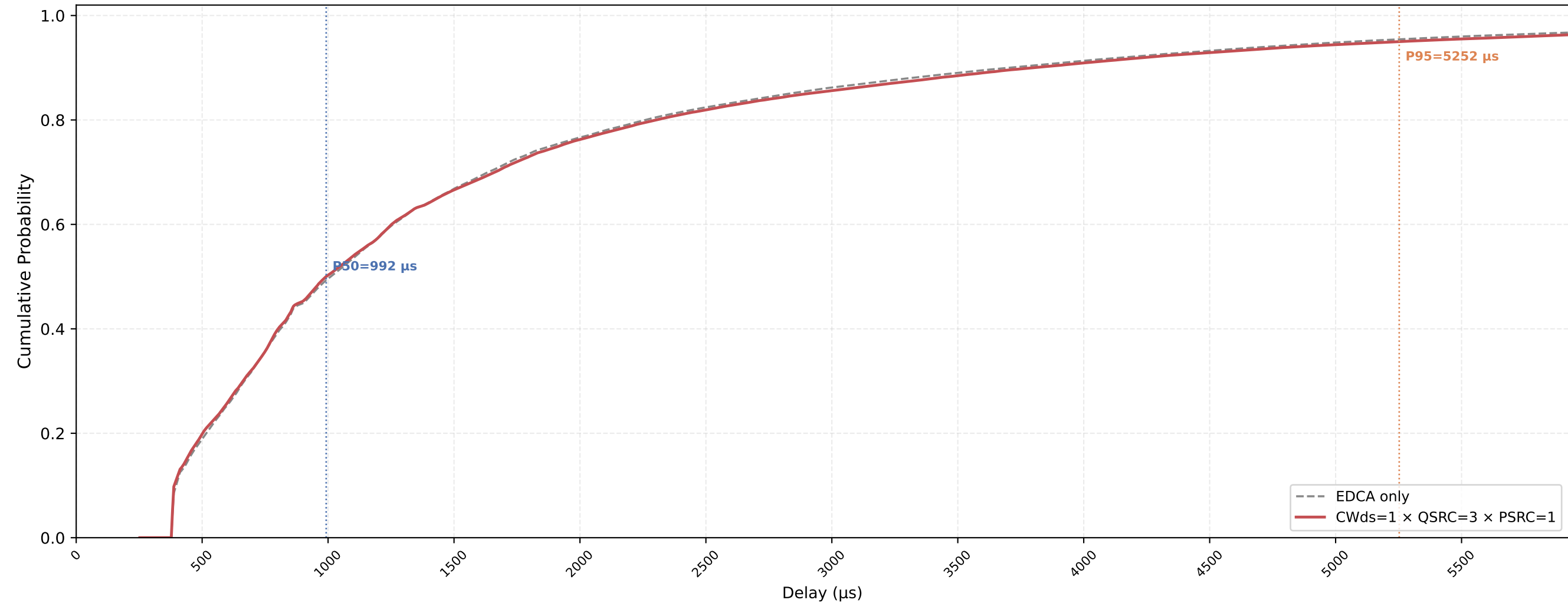
Legacy STA VO Delay CDF — CWds=1 × QSRC=3 × PSRC=1 nSta=30, nPedca=15, 0.5Mbps, avg of 10 runs
