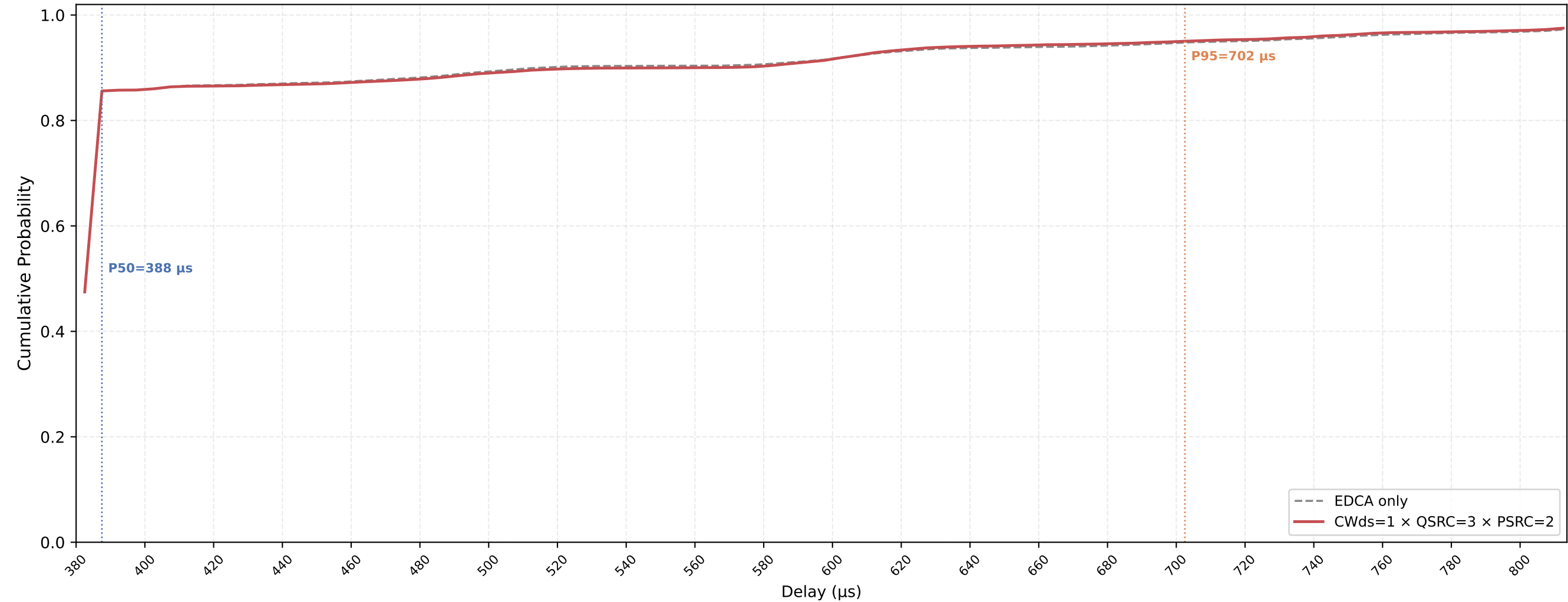
Legacy STA VO Delay CDF — CWds=1 × QSRC=3 × PSRC=2 nSta=30, nPedca=5, 0.1Mbps, avg of 10 runs
