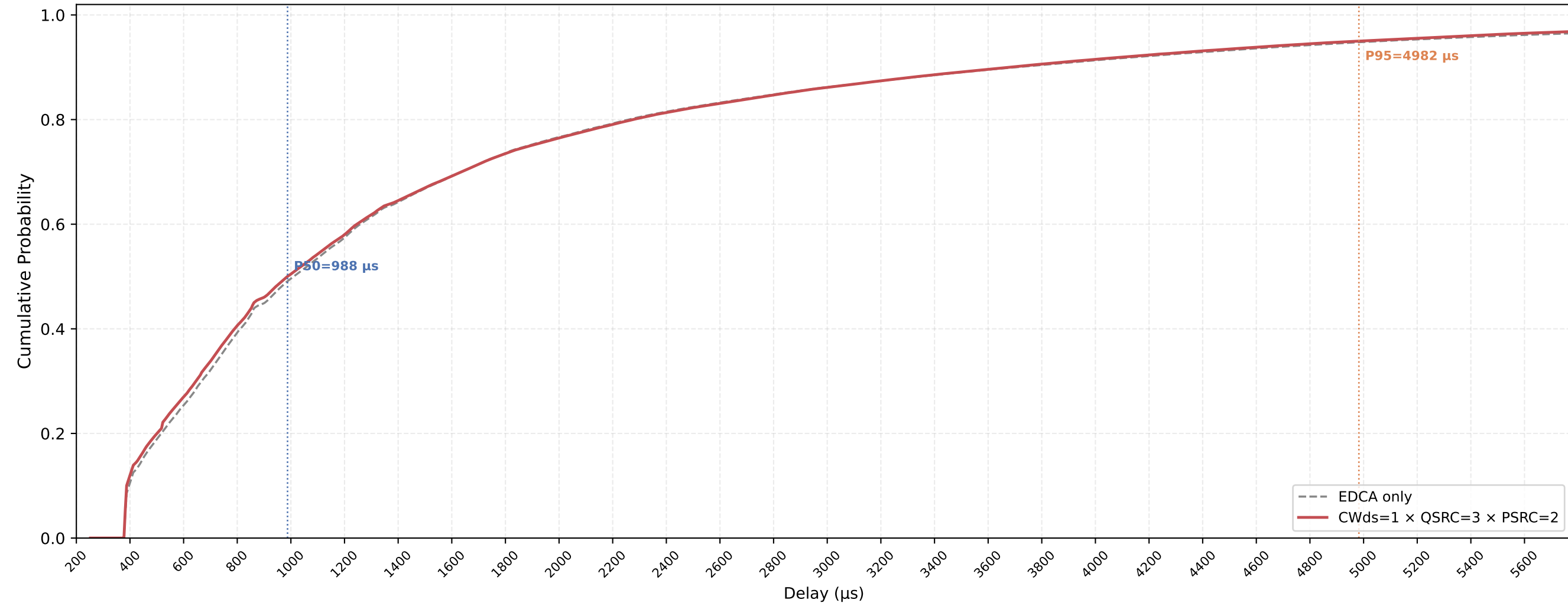
P-EDCA STA VO Delay CDF — CWds=1 × QSRC=3 × PSRC=2 nSta=30, nPedca=30, 0.5Mbps, avg of 10 runs
