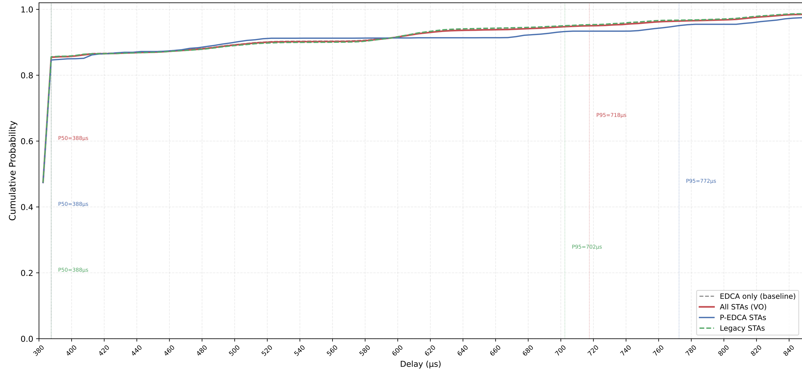
VO Delay CDF — P-EDCA / Legacy / All | CWds=1 × QSRC=3 × PSRC=3 nSta=30, nPedca=5/30, 0.1Mbps, avg of 10 runs
