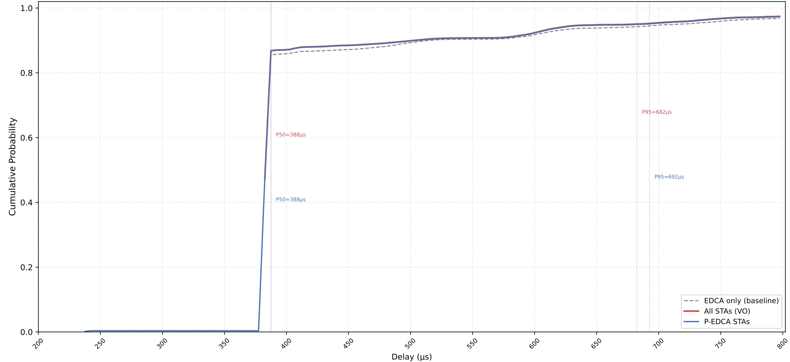
VO Delay CDF — P-EDCA / Legacy / All | CWds=1 × QSRC=3 × PSRC=3 nSta=30, nPedca=30/30, 0.1Mbps, avg of 10 runs
