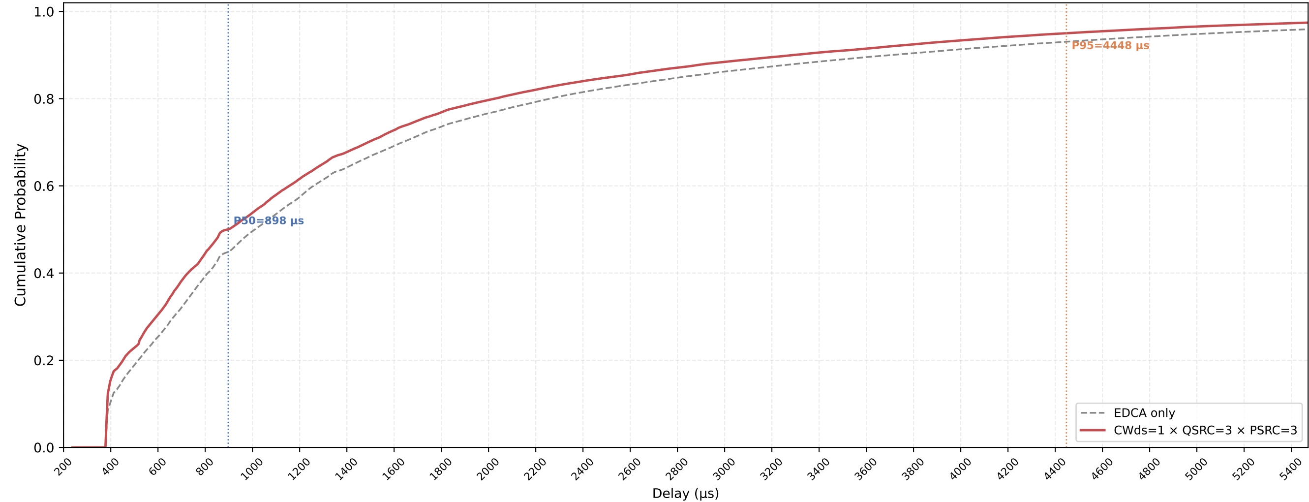
P-EDCA STA VO Delay CDF — CWds=1 × QSRC=3 × PSRC=3 nSta=30, nPedca=15, 0.5Mbps, avg of 10 runs
