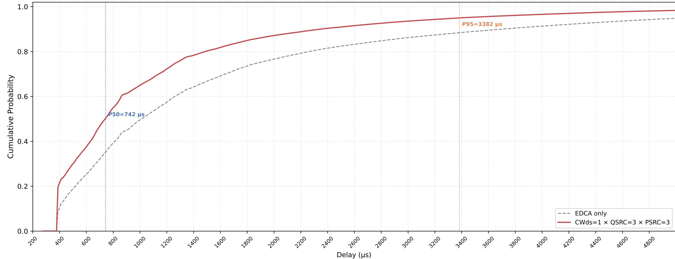
VO (all STAs) Delay CDF — CWds=1 × QSRC=3 × PSRC=3 nSta=30, nPedca=30, 0.5Mbps, avg of 10 runs
