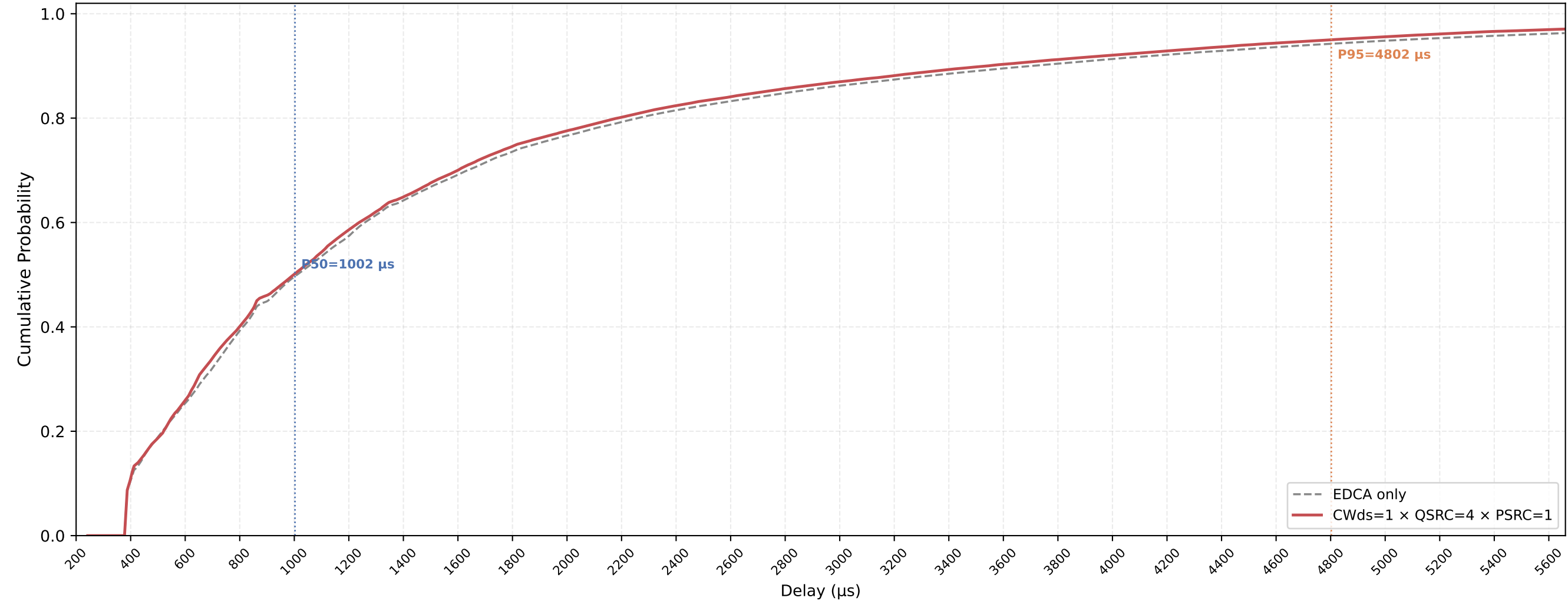
P-EDCA STA VO Delay CDF — CWds=1 × QSRC=4 × PSRC=1 nSta=30, nPedca=15, 0.5Mbps, avg of 10 runs
