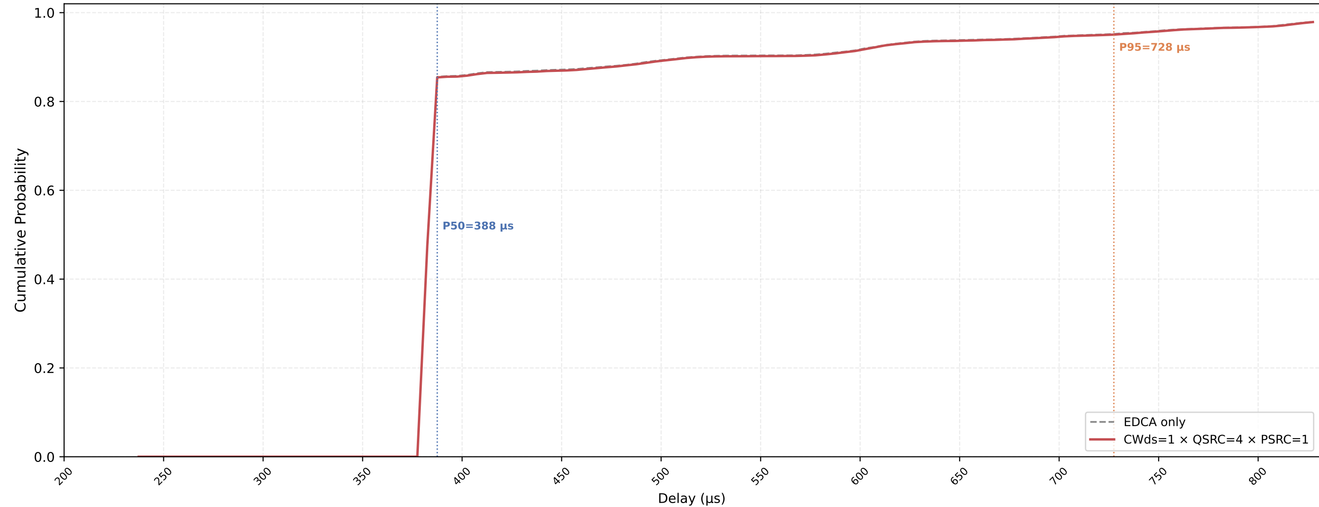
P-EDCA STA VO Delay CDF — CWds=1 × QSRC=4 × PSRC=1 nSta=30, nPedca=30, 0.1Mbps, avg of 10 runs
