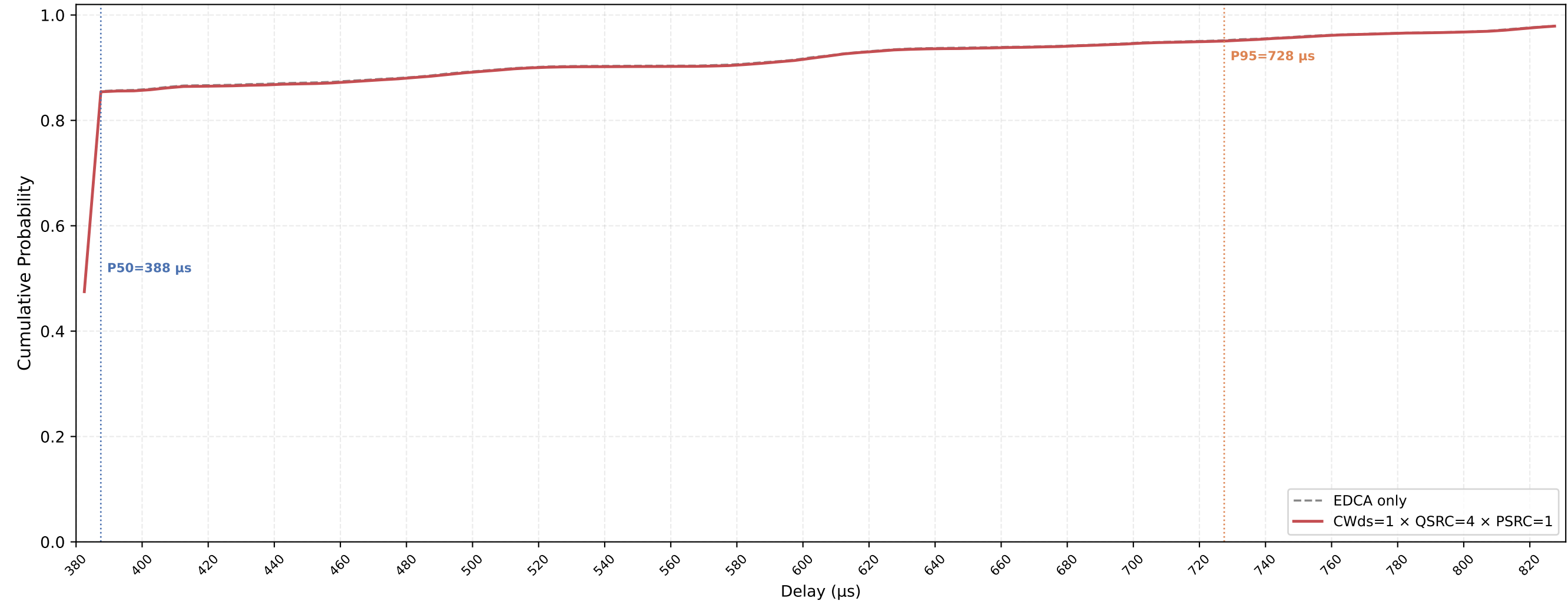
VO (all STAs) Delay CDF — CWds=1 × QSRC=4 × PSRC=1 nSta=30, nPedca=30, 0.1Mbps, avg of 10 runs
