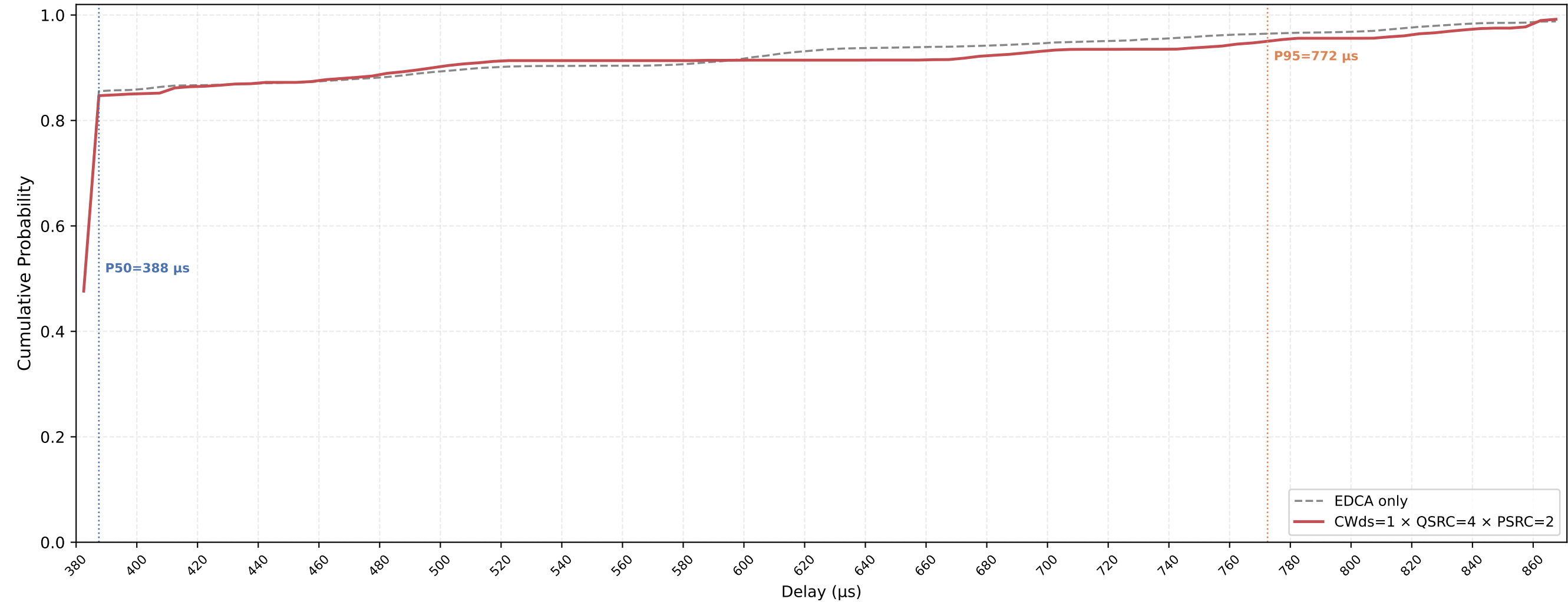
P-EDCA STA VO Delay CDF — CWds=1 × QSRC=4 × PSRC=2 nSta=30, nPedca=5, 0.1Mbps, avg of 10 runs
