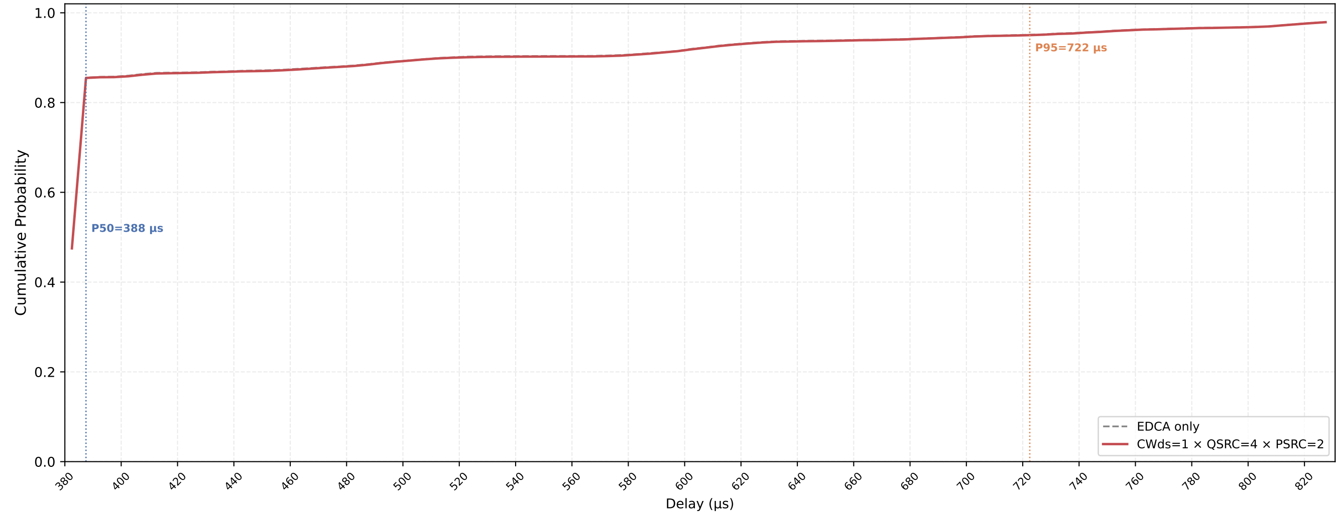
VO (all STAs) Delay CDF — CWds=1 × QSRC=4 × PSRC=2 nSta=30, nPedca=15, 0.1Mbps, avg of 10 runs
