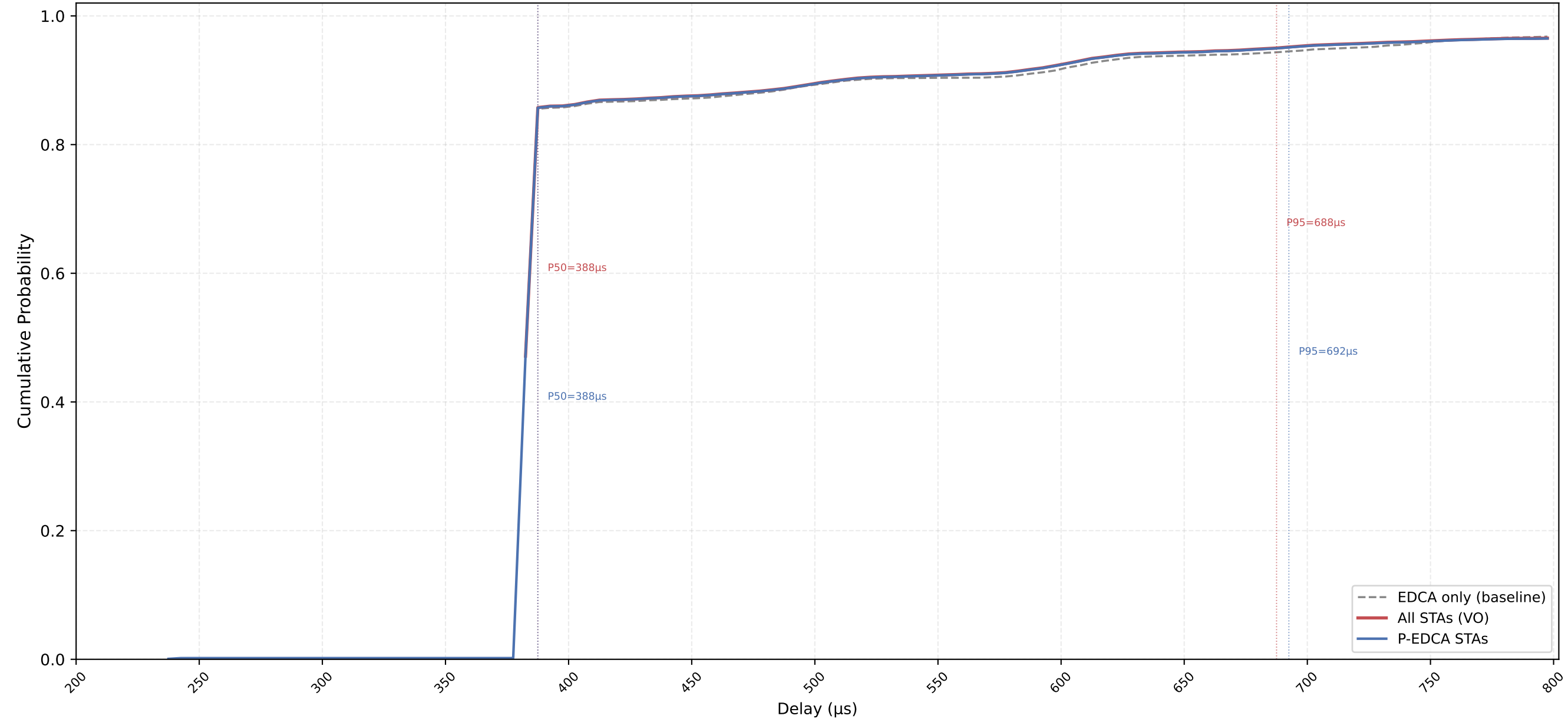
VO Delay CDF — P-EDCA / Legacy / All | CWds=1 × QSRC=4 × PSRC=3 nSta=30, nPedca=30/30, 0.1Mbps, avg of 10 runs
