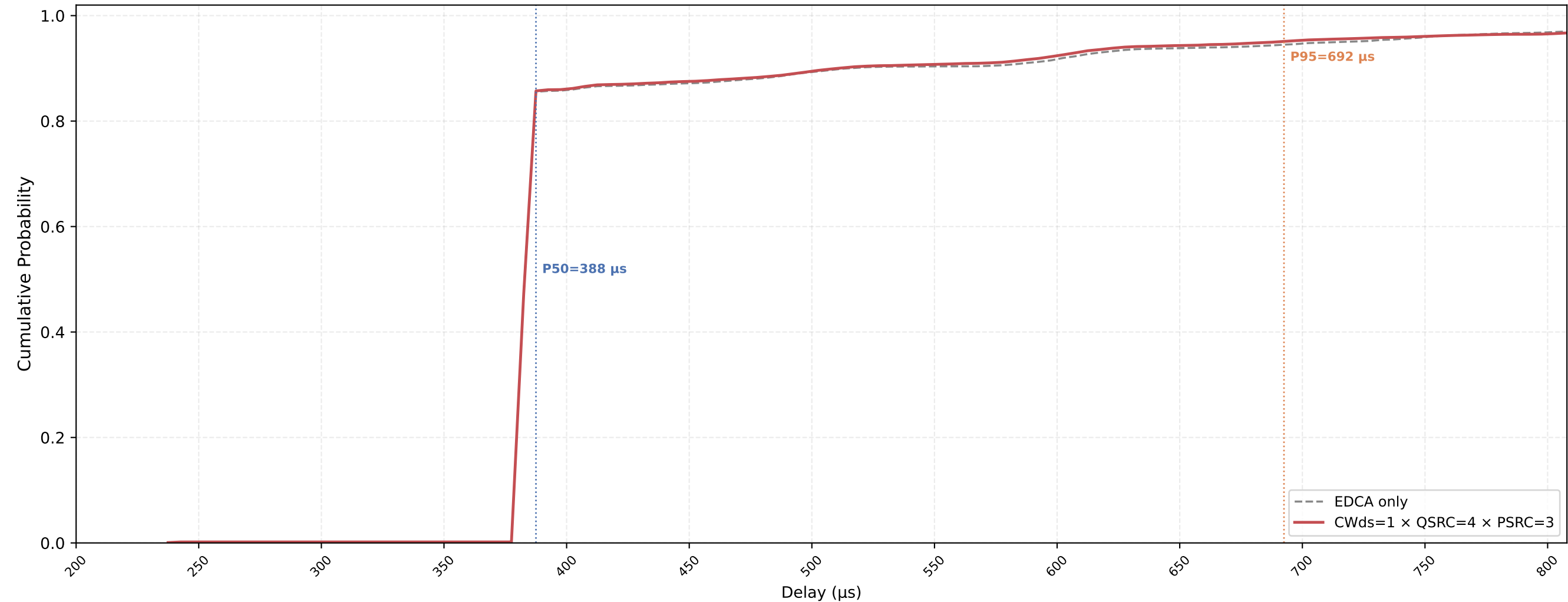
P-EDCA STA VO Delay CDF — CWds=1 × QSRC=4 × PSRC=3 nSta=30, nPedca=30, 0.1Mbps, avg of 10 runs
