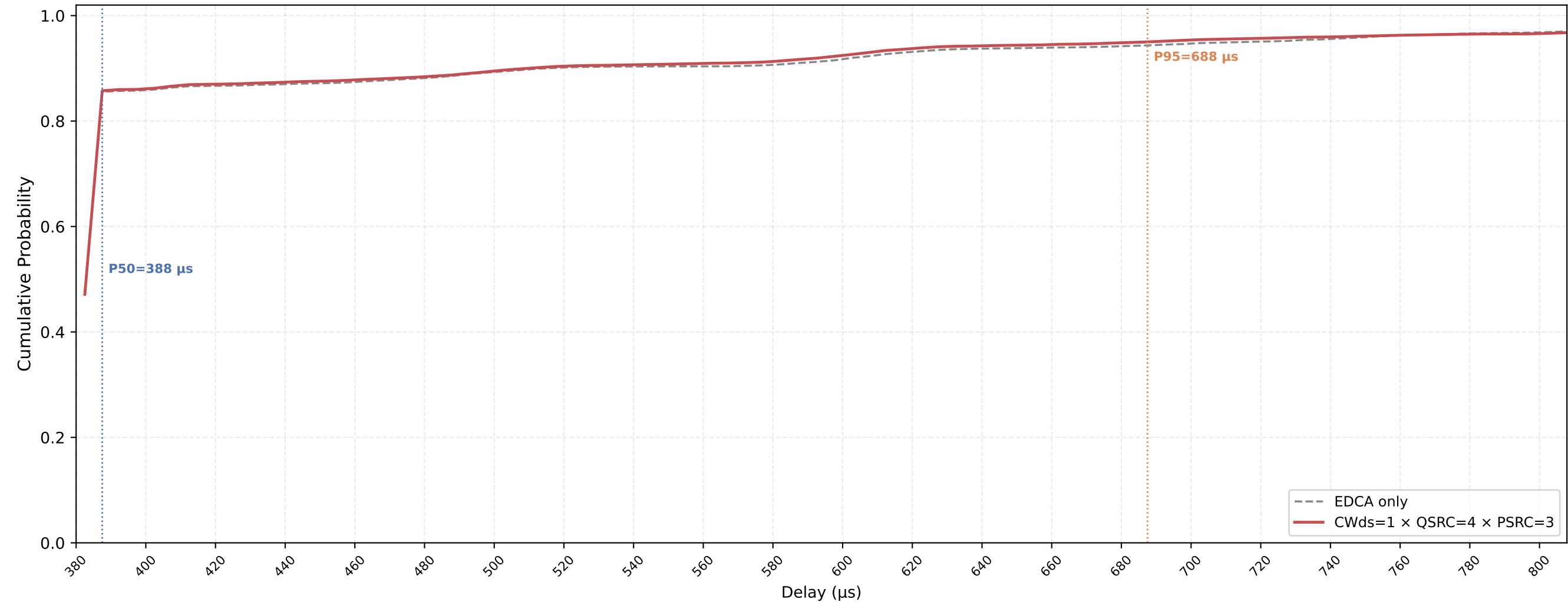
VO (all STAs) Delay CDF — CWds=1 × QSRC=4 × PSRC=3 nSta=30, nPedca=30, 0.1Mbps, avg of 10 runs
