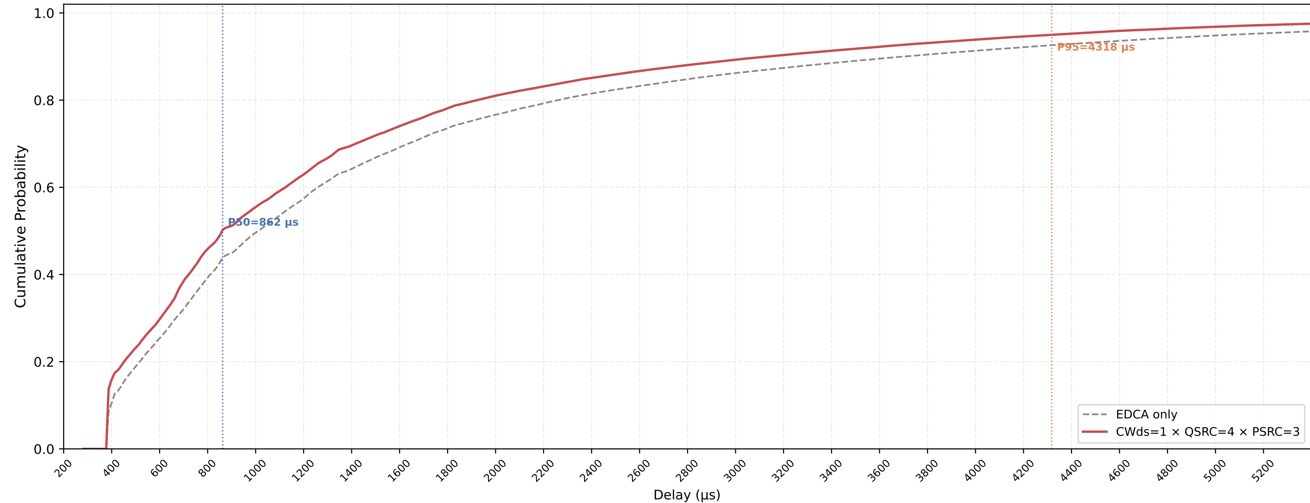
VO (all STAs) Delay CDF — CWds=1 × QSRC=4 × PSRC=3 nSta=30, nPedca=30, 0.5Mbps, avg of 10 runs
