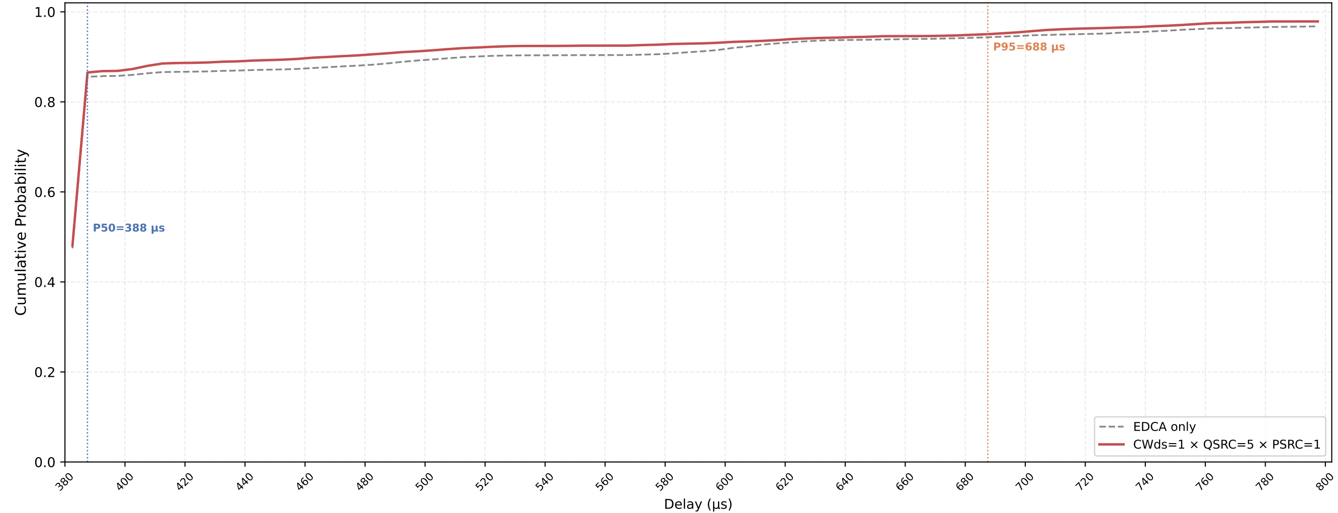
P-EDCA STA VO Delay CDF — CWds=1 × QSRC=5 × PSRC=1 nSta=30, nPedca=15, 0.1Mbps, avg of 10 runs
