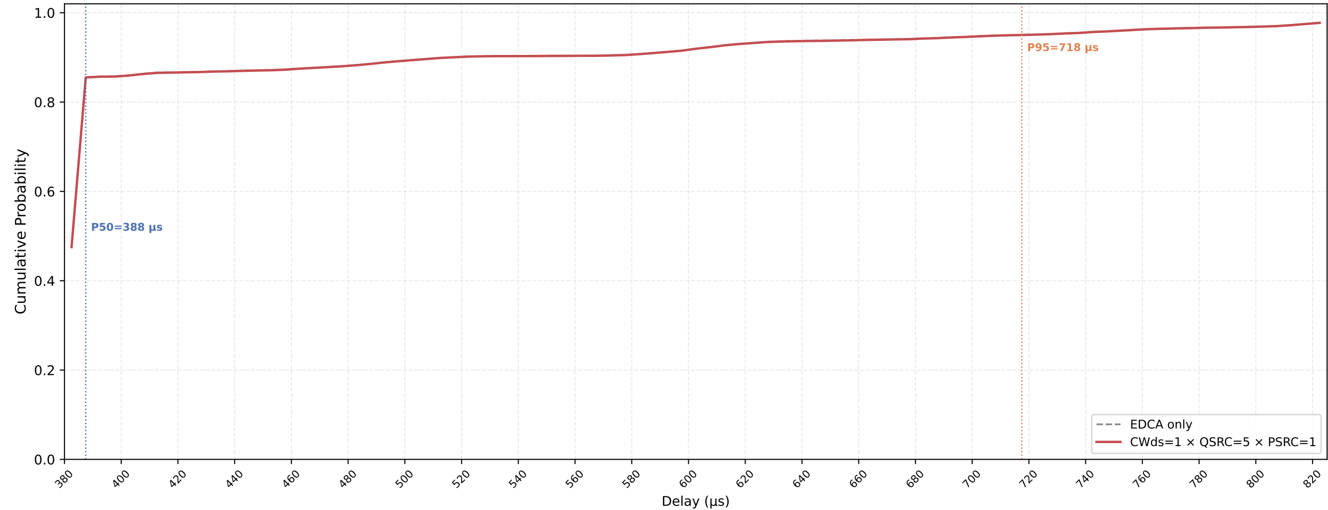
VO (all STAs) Delay CDF — CWds=1 × QSRC=5 × PSRC=1 nSta=30, nPedca=15, 0.1Mbps, avg of 10 runs
