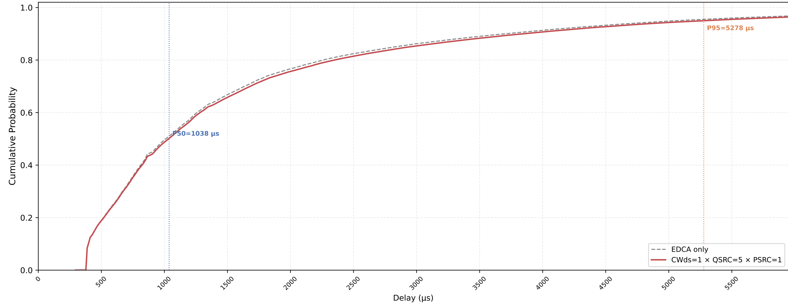
VO (all STAs) Delay CDF — CWds=1 × QSRC=5 × PSRC=1 nSta=30, nPedca=15, 0.5Mbps, avg of 10 runs
