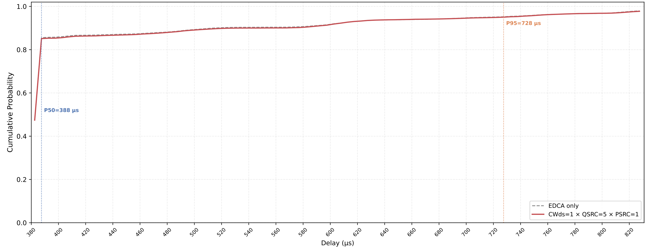
VO (all STAs) Delay CDF — CWds=1 × QSRC=5 × PSRC=1 nSta=30, nPedca=30, 0.1Mbps, avg of 10 runs
