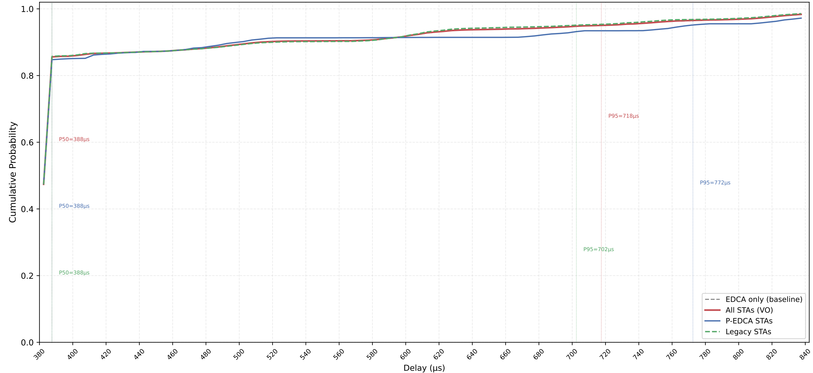
VO Delay CDF — P-EDCA / Legacy / All | CWds=1 × QSRC=5 × PSRC=2 nSta=30, nPedca=5/30, 0.1Mbps, avg of 10 runs
