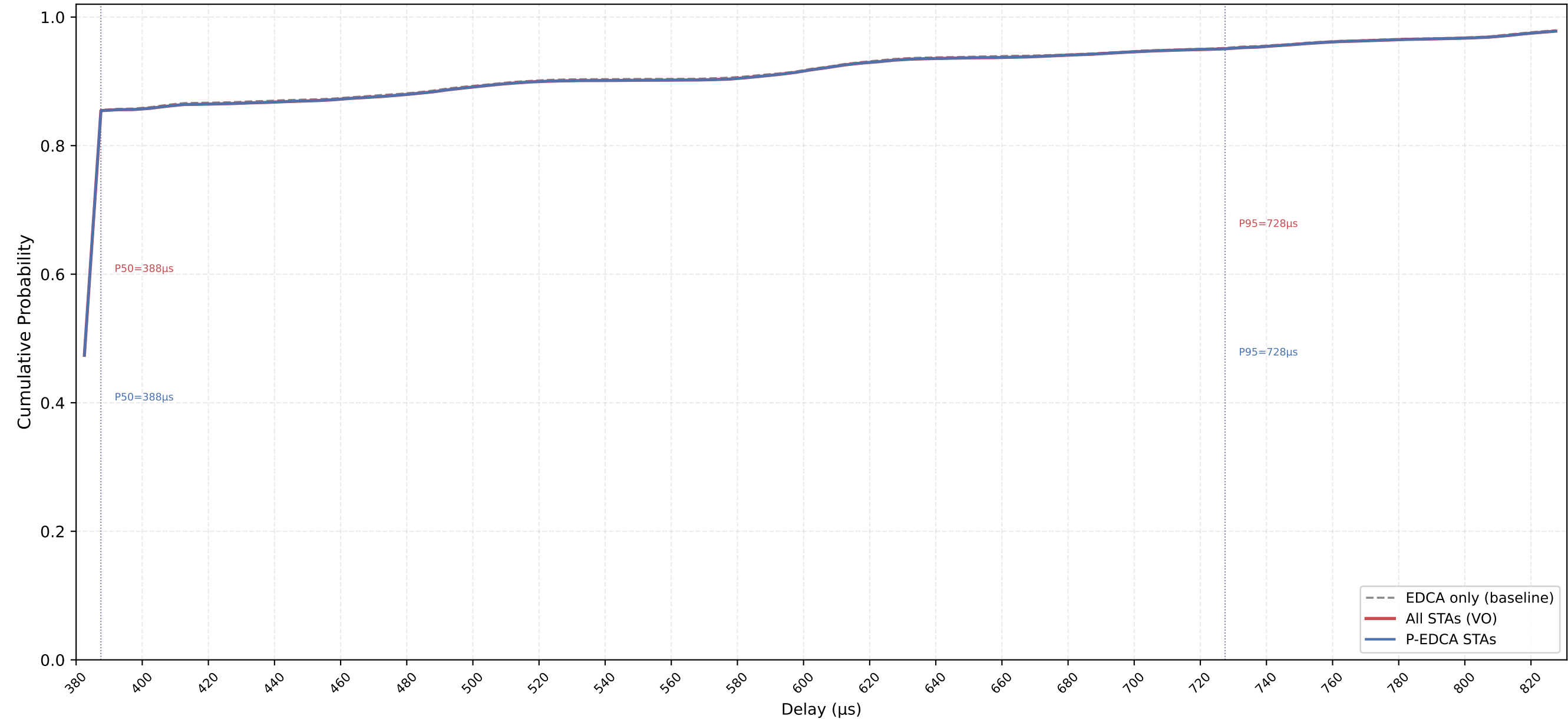
VO Delay CDF — P-EDCA / Legacy / All | CWds=1 × QSRC=5 × PSRC=2 nSta=30, nPedca=30/30, 0.1Mbps, avg of 10 runs
