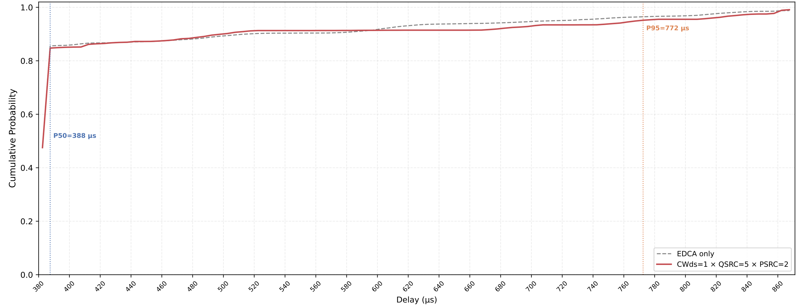
P-EDCA STA VO Delay CDF — CWds=1 × QSRC=5 × PSRC=2 nSta=30, nPedca=5, 0.1Mbps, avg of 10 runs
