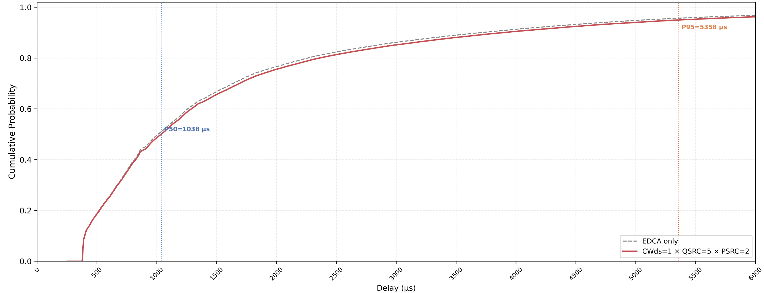
P-EDCA STA VO Delay CDF — CWds=1 × QSRC=5 × PSRC=2 nSta=30, nPedca=30, 0.5Mbps, avg of 10 runs
