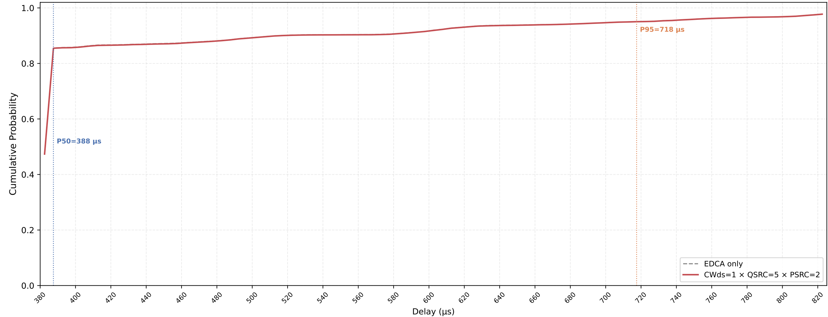
VO (all STAs) Delay CDF — CWds=1 × QSRC=5 × PSRC=2 nSta=30, nPedca=15, 0.1Mbps, avg of 10 runs
