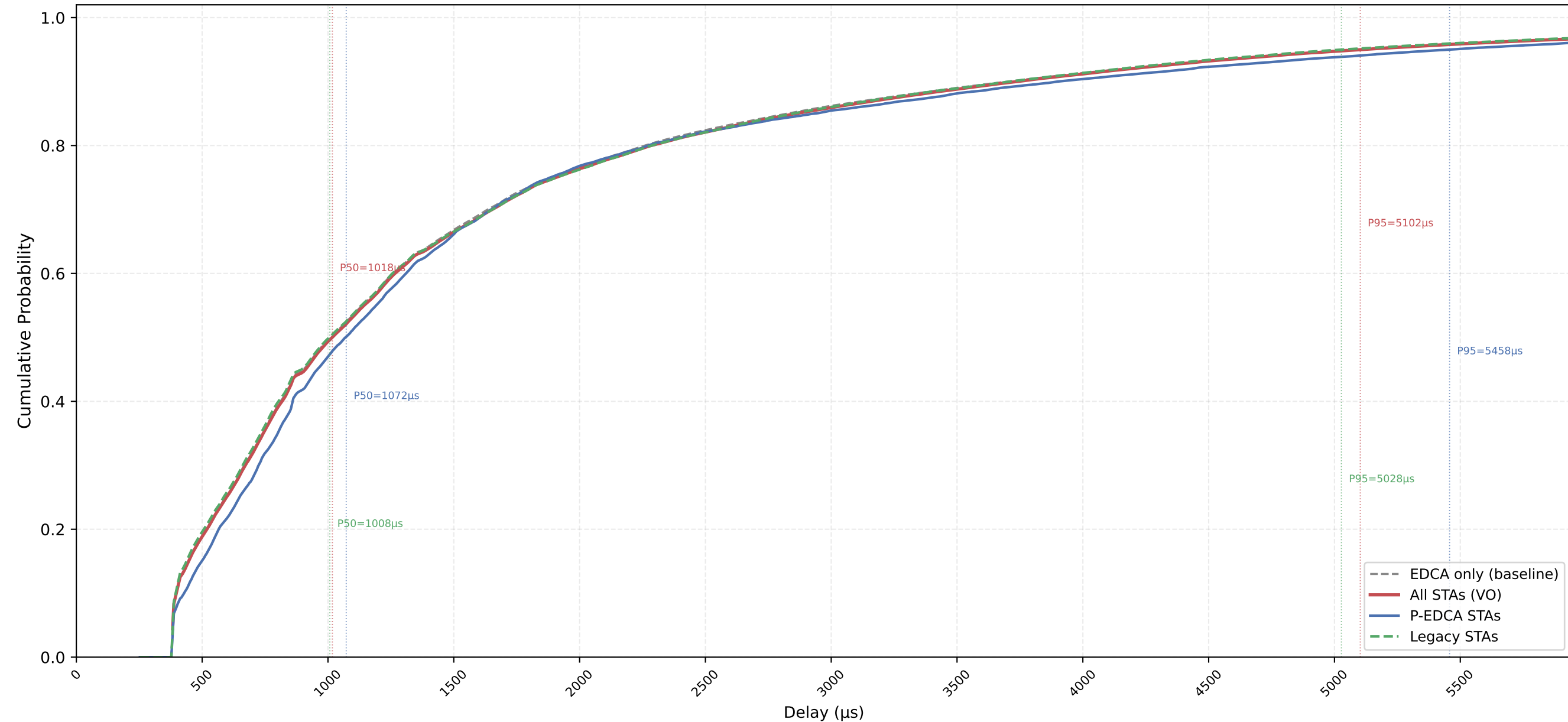
VO Delay CDF — P-EDCA / Legacy / All | CWds=1 × QSRC=5 × PSRC=3 nSta=30, nPedca=5/30, 0.5Mbps, avg of 10 runs
