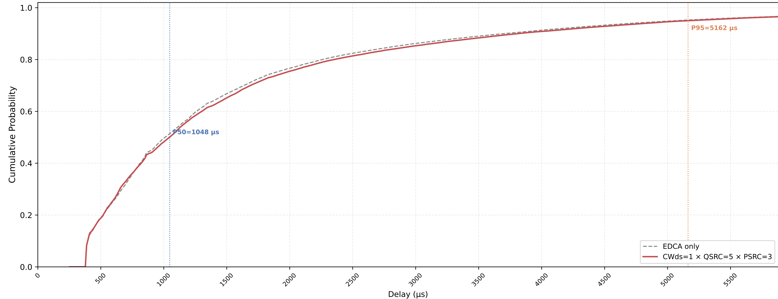
P-EDCA STA VO Delay CDF — CWds=1 × QSRC=5 × PSRC=3 nSta=30, nPedca=15, 0.5Mbps, avg of 10 runs
