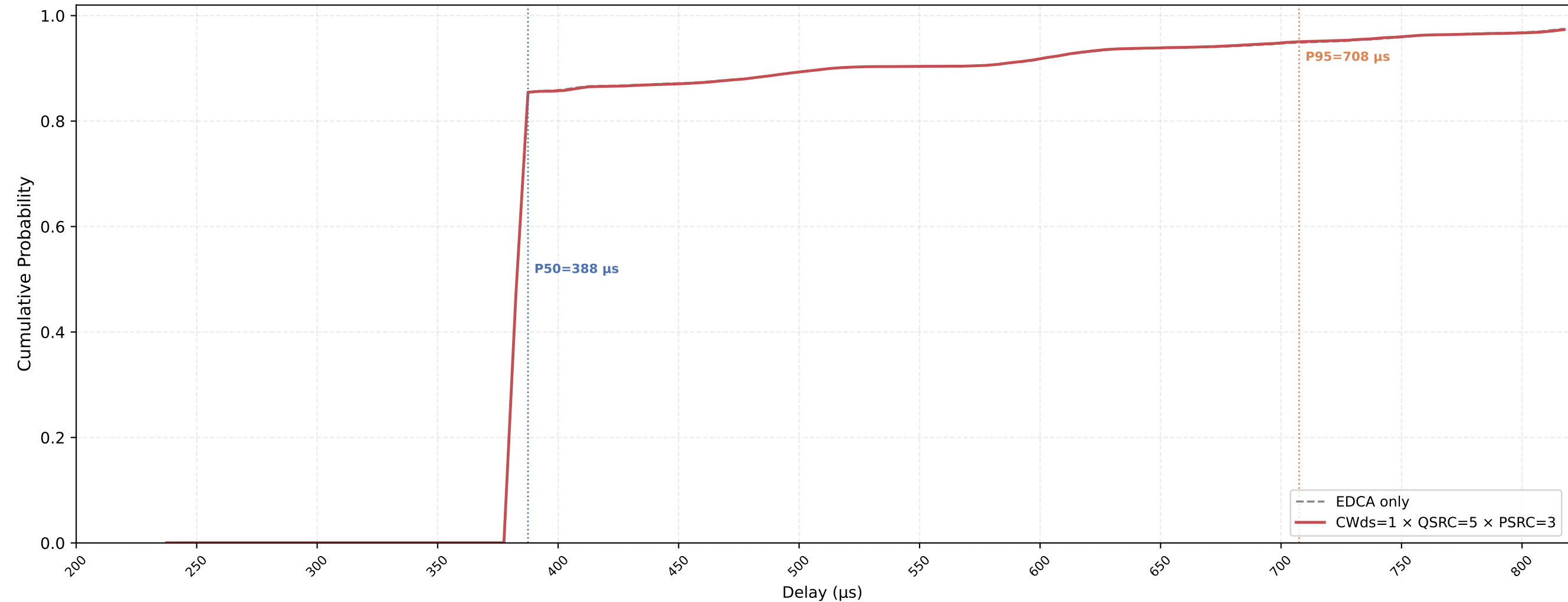
P-EDCA STA VO Delay CDF — CWds=1 × QSRC=5 × PSRC=3 nSta=30, nPedca=30, 0.1Mbps, avg of 10 runs
