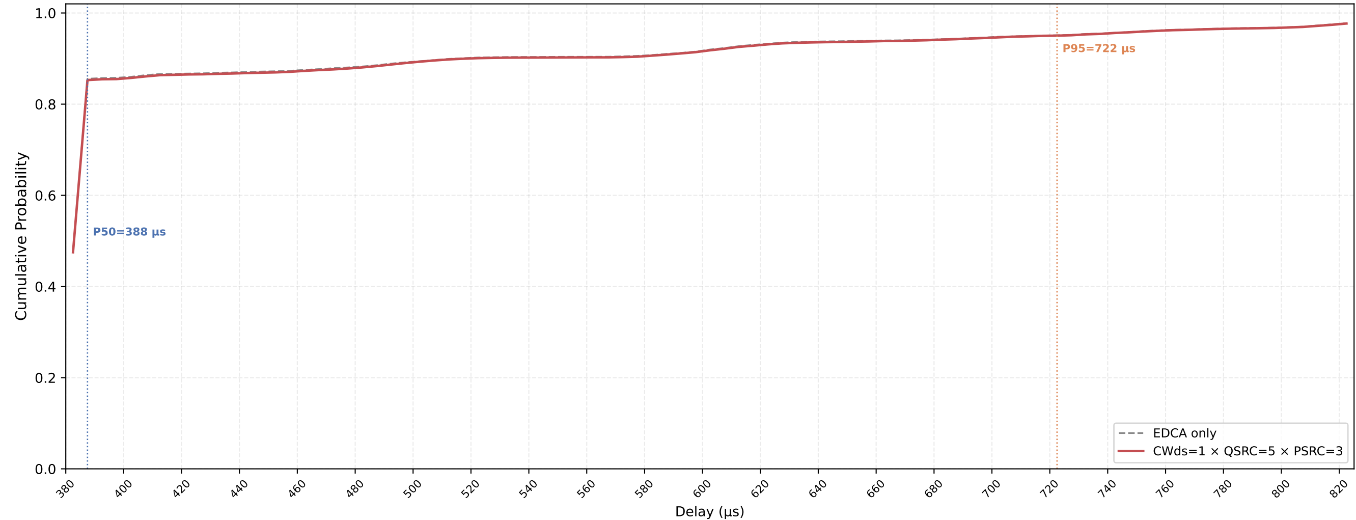
VO (all STAs) Delay CDF — CWds=1 × QSRC=5 × PSRC=3 nSta=30, nPedca=15, 0.1Mbps, avg of 10 runs
