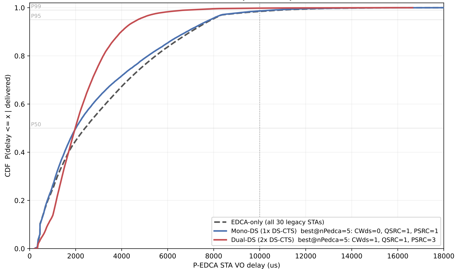
P-EDCA STA Delay CDF at Best Parameters (nPedca=5/30, nSta=30, 1Mbps) curves normalised to 1.0 — delay SHAPE only, loss not shown
