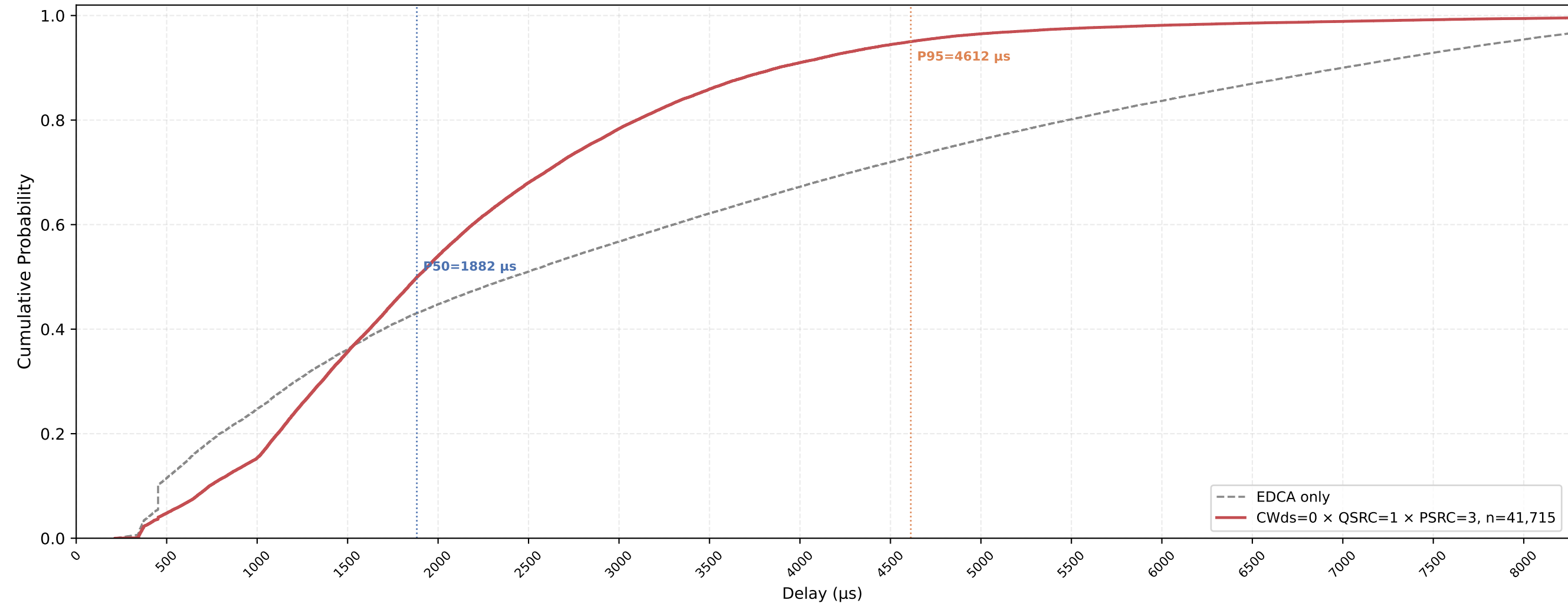
P-EDCA STA VO Delay CDF — CWds=0 × QSRC=1 × PSRC=3 nSta=30, nPedca=5, 1Mbps, avg of 10 runs
